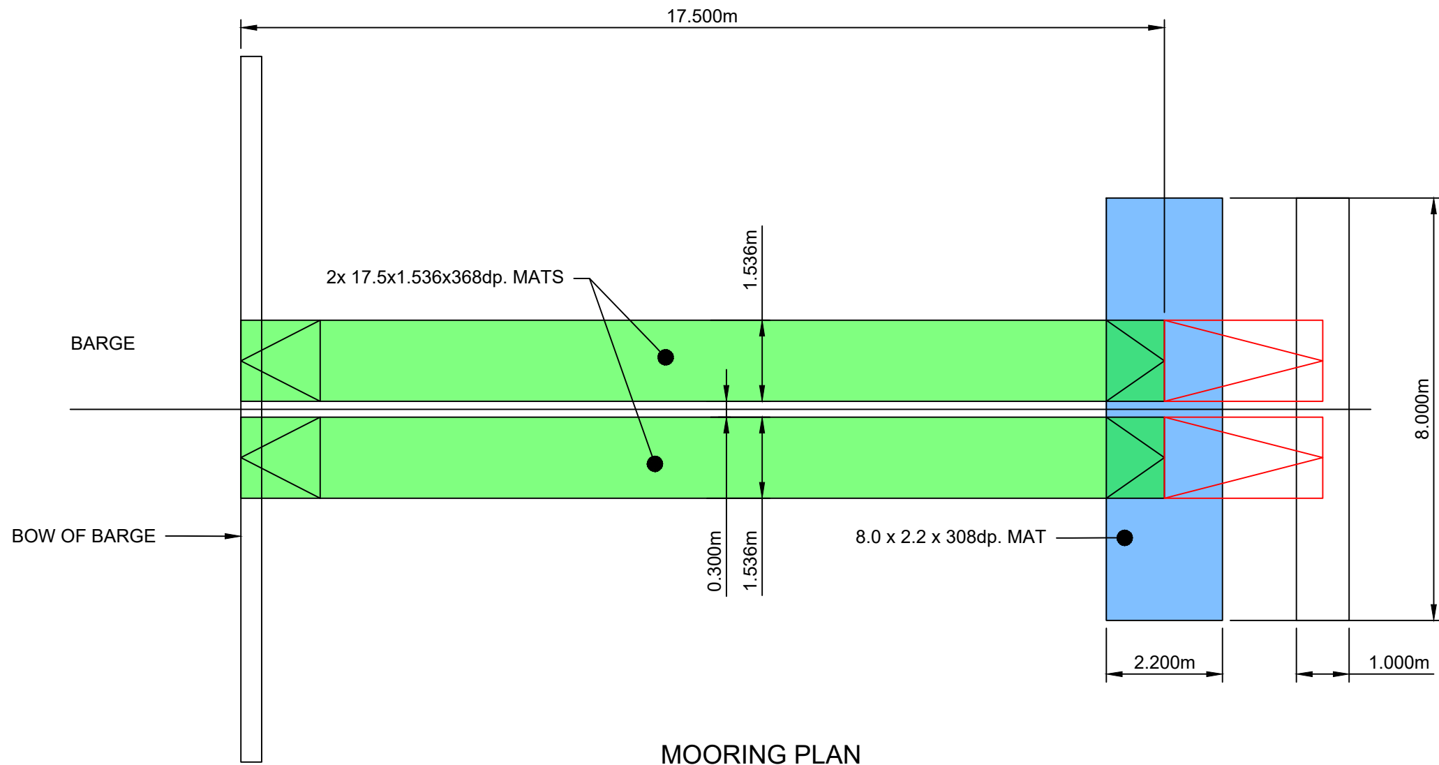
MOORING PLAN (SCALE 1:100)
